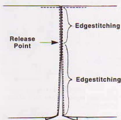
Fig. 6-8. Inverted pleat edgestitched \frac{1}{16} " (1.5mm) from the folds through three layers to lower the release point, and through two layers to crease the pleat folds permanently.
