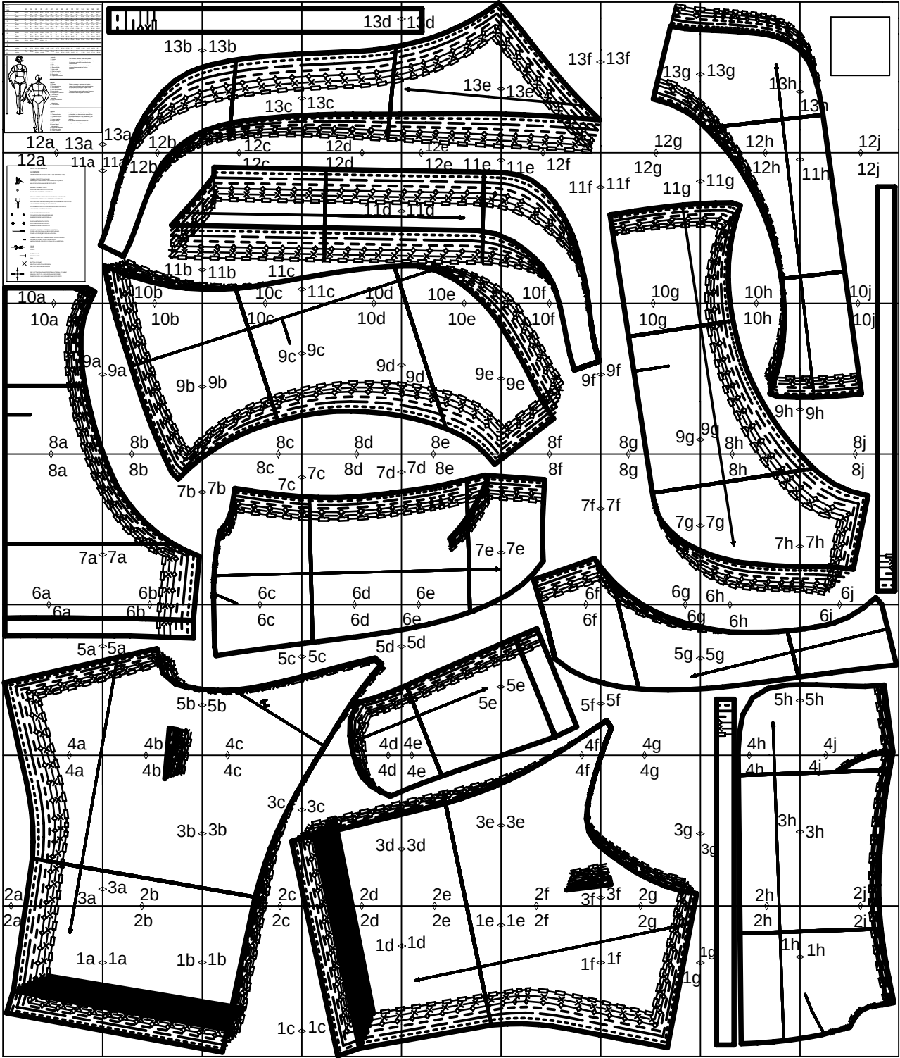
layout drawing
