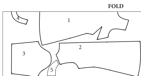
Layplan for 60"-wide fabric all sizes
